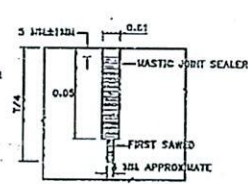
DETAIL "A" (CONTRACTION JOINT)
