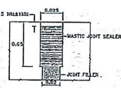
DETAIL "C" (EXPANSION JOINT)
