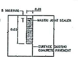
DETAIL "B" (CONSTRUCTION JOINT)
