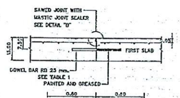
DETAIL OF CONSTRUCTION JOINT NOT TO SACLE
